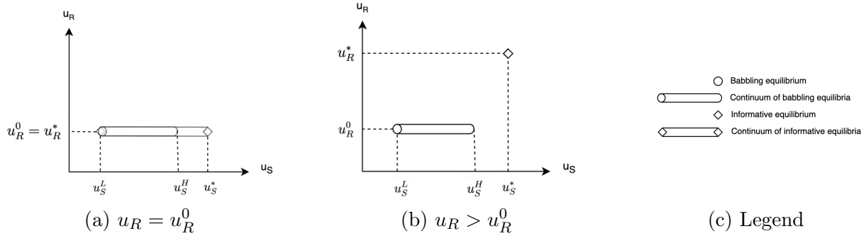
Figure 3: Possible PBE payoffs when there exists an informative PBE \sigma with payoff profile (u_S, u_R) . Example games that generate such payoffs can be found in Figure 18 in the Appendix. Note that Figure 3a and 3b cannot happen at the same time, which is shown in Theorem 6 in the Appendix.
