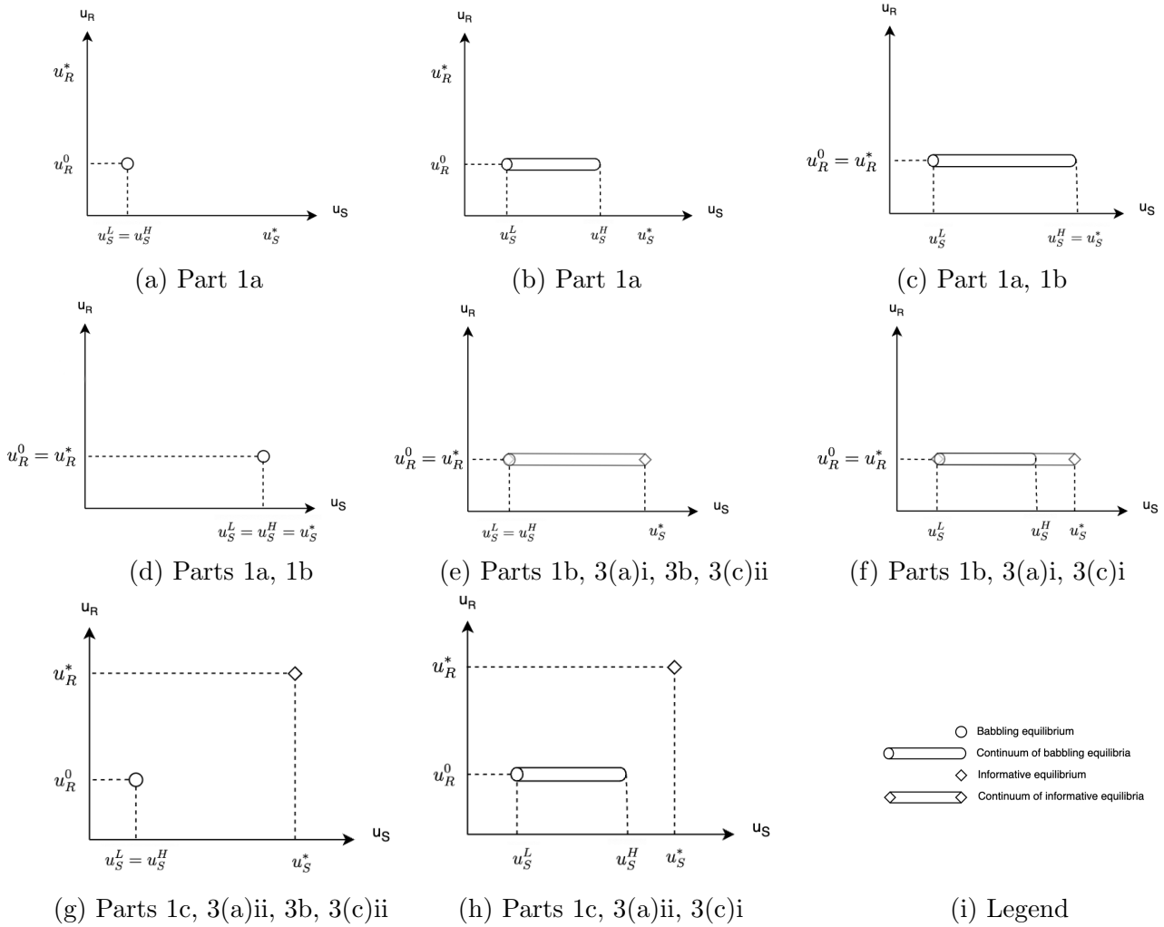
Figure 15: Possible PBE payoffs for binary action cheap talk games, with the relevant parts of Theorem 6 listed. Note that part 2 applies to all examples. Example games that generate such payoffs can be found in Figure 18 in the Appendix.
